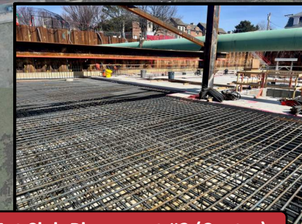
Rebar for Mat Slab Placement #2 (Center)
