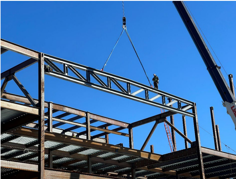
The first roof truss being installed over the roof on February 8, 2024.
