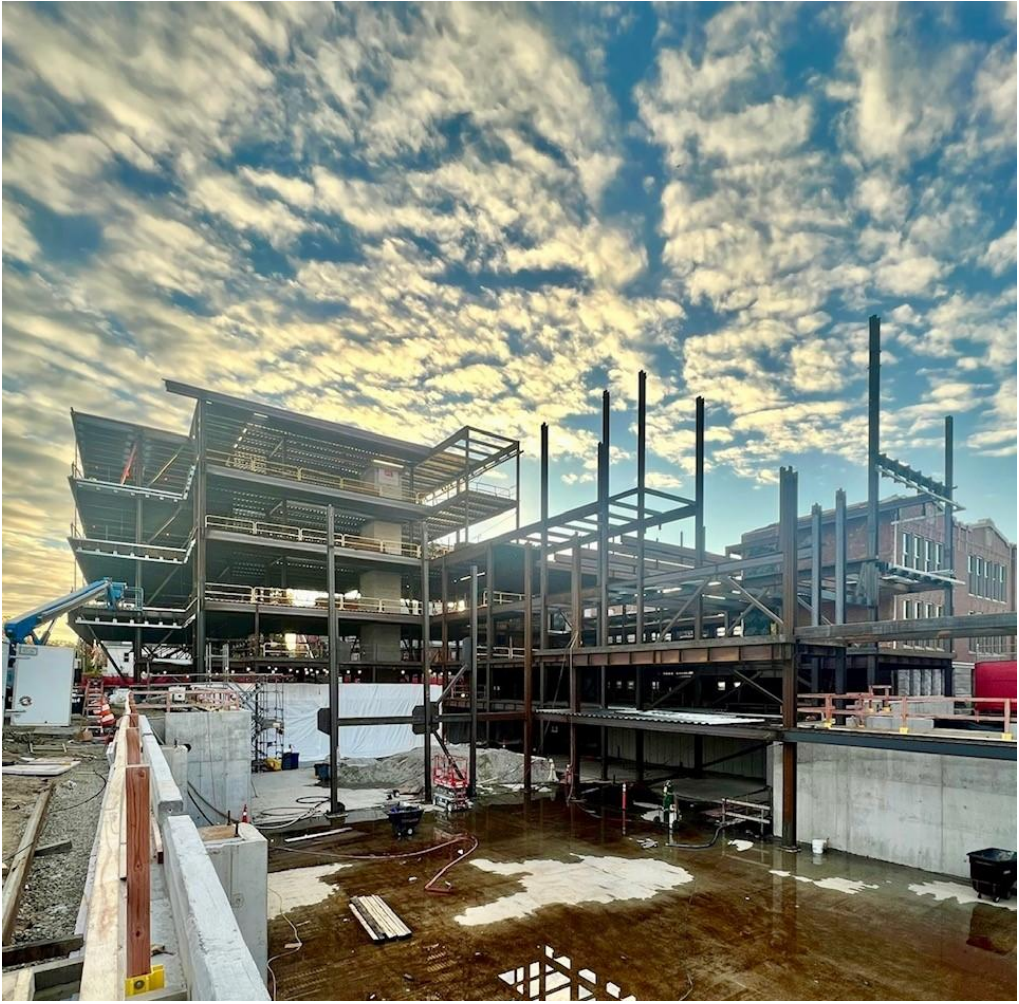
Steel Erection Complete – East Half
